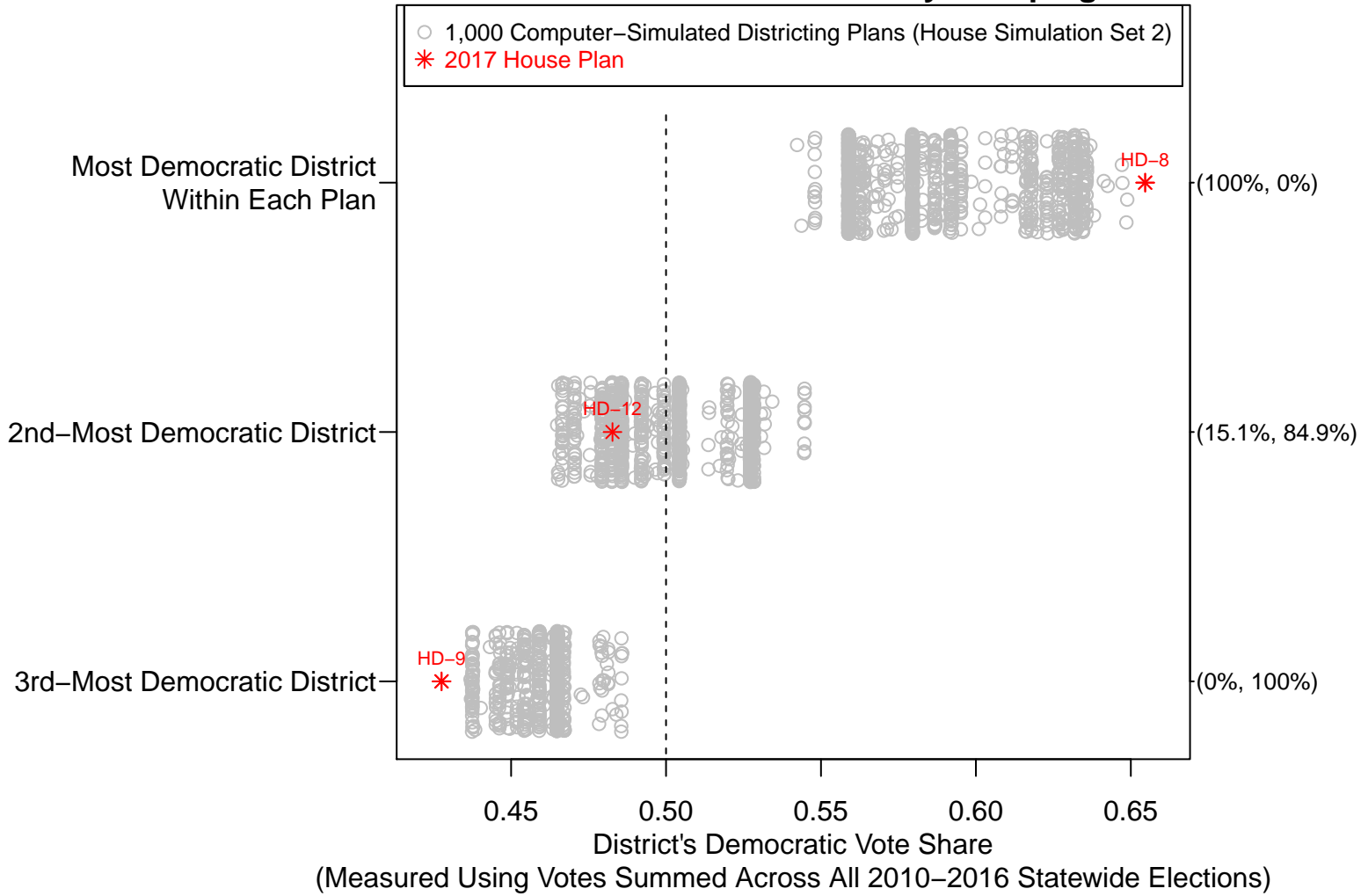
Figure 44: House Simulation Set 2: Democratic Vote Share of the Enacted and Computer-Simulated Districts Within the Lenoir-Pitt County Grouping
