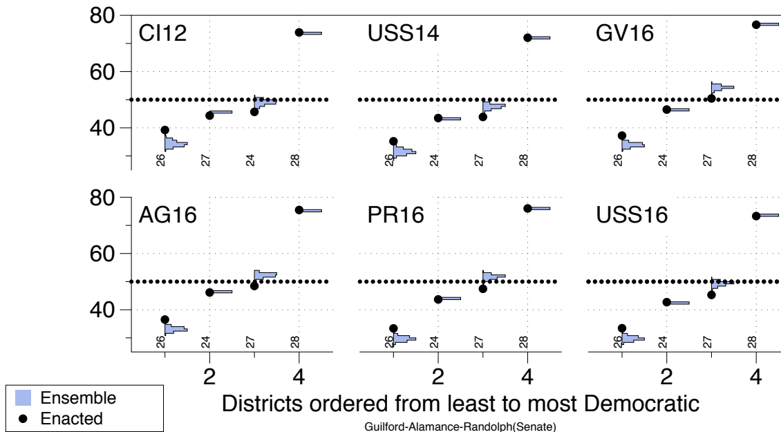
Figure 20: The districts in each plan of the ensemble are ordered from least to most Democratic for a given election. The results found in the ensemble of plans are contrasted with the enacted plan; the actual district numbers of the enacted plan are given.
