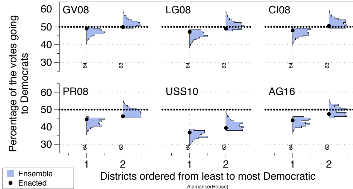
Figure 24: The districts in each plan of the ensemble are ordered from least to most Democratic for a given election. The results found in the ensemble of plans are contrasted with the enacted plan; the actual district numbers of the enacted plan are given.
