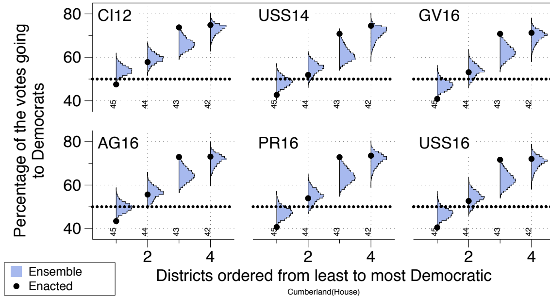
Figure 30: The districts in each plan of the ensemble are ordered from least to most Democratic for a given election. The results found in the ensemble of plans are contrasted with the enacted plan; the actual district numbers of the enacted plan are given.
