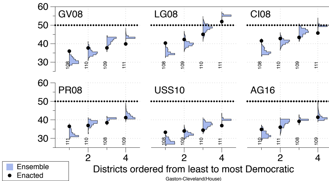
Figure 36: The districts in each plan of the ensemble are ordered from least to most Democratic for a given election. The results found in the ensemble of plans are contrasted with the enacted plan; the actual district numbers of the enacted plan are given.
