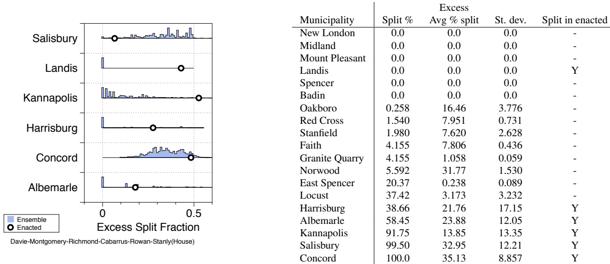
Figure 78: We compare municipal divisions of the enacted plan with the ensemble. Split % reports the fraction of plans in the ensemble in which the given municipality was split. Avg. Split reports the fraction of the population that was removed from the core district(s) and St. dev. is the standard deviation of this split in the ensemble.
