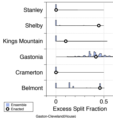
Figure 82: We compare municipal divisions of the enacted plan with the ensemble. Split % reports the fraction of plans in the ensemble in which the given municipality was split. Avg. Split reports the fraction of the population that was removed from the core district(s) and St. dev. is the standard deviation of this split in the ensemble.
