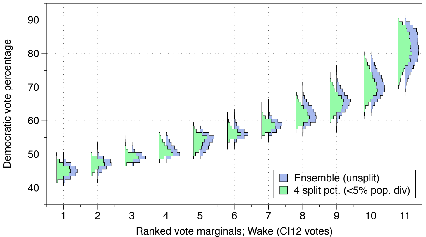
Figure 101: We plot ranked marginal distributions in the ensemble of House districts for Mecklenburg (left) and Wake (right). We compare our original distribution that does not split precincts, with the plans from the ensemble that have been altered to achieve compliant population deviation and split fewer than four precincts. In Mecklenburg, we also display the collection of split-precinct plans that split 3 or fewer precincts.
