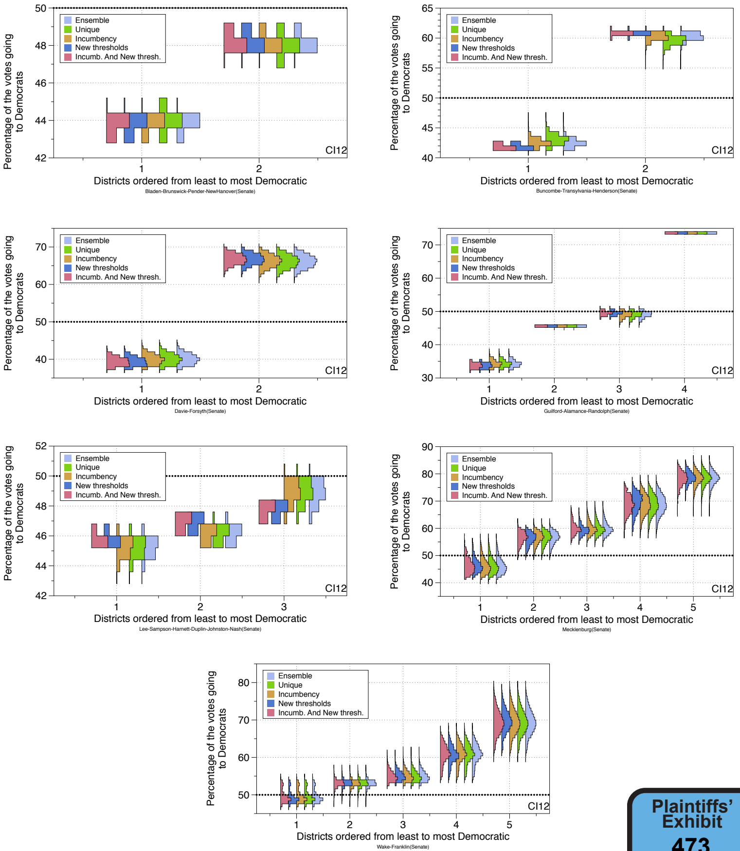
Figure 104: We examine the difference in the marginal distributions when considering incumbency, reweighting the space, and having more stringent redistricting criteria. We examine the Senate clusters presented in Section 4
